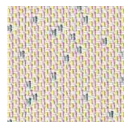
Milkyway powder
