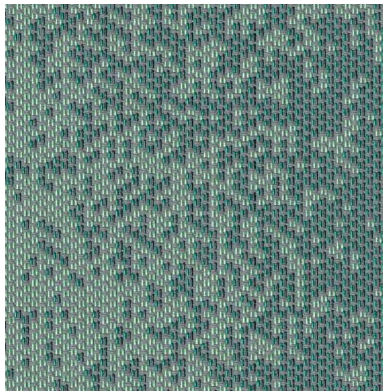
Milkyway jade
