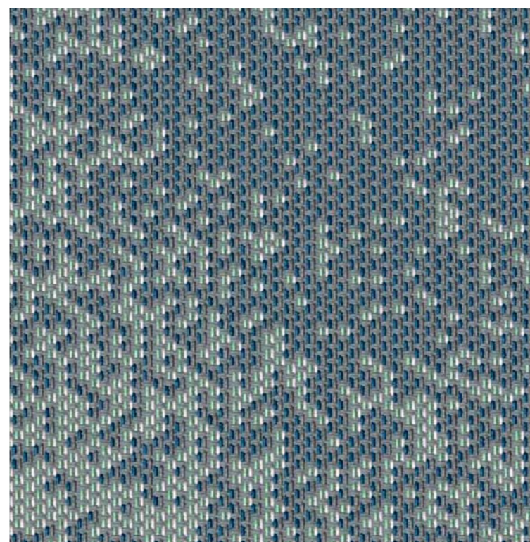
Milkyway shadow
