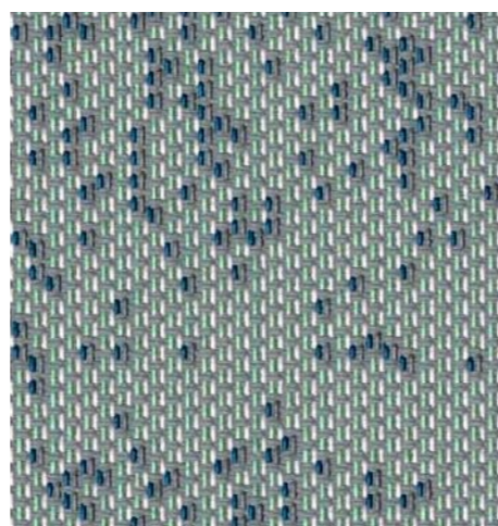
Milkyway shadow
