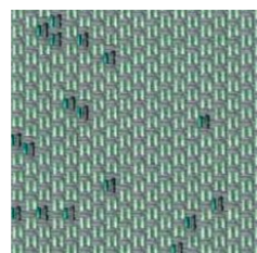
Milkyway jade
