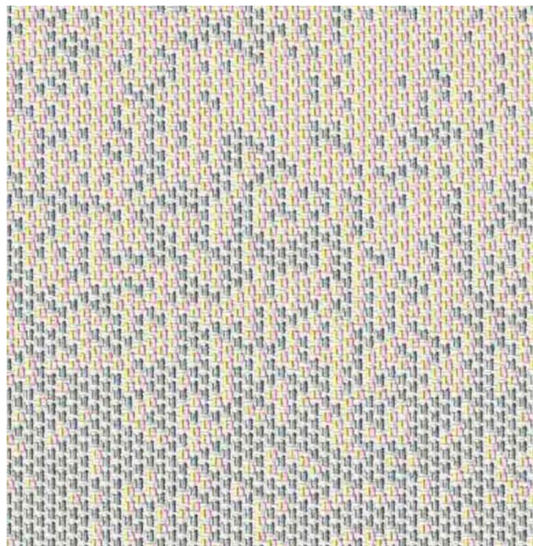
Milkyway powder
