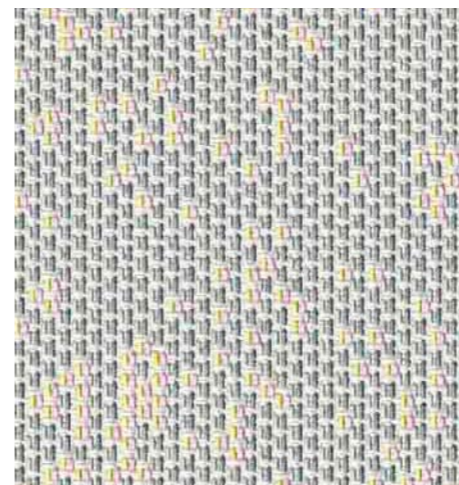
Milkyway powder
