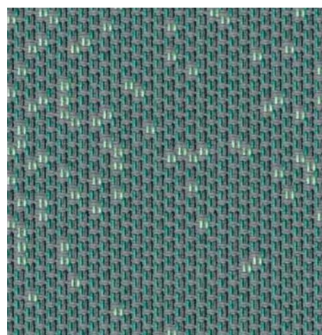
Milkyway jade
